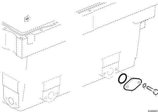
SEAL ELEM. 010.00140
