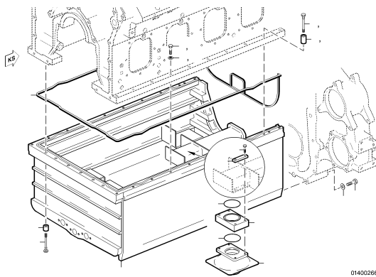
OIL PAN 010.00130
